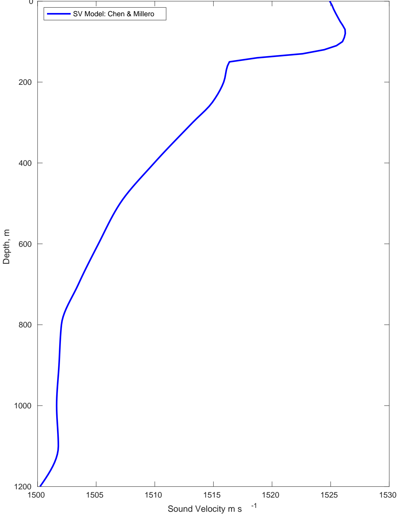
Sound Velocity Profile for Las Palmas Yard on 02-May-2024 00:00:00
